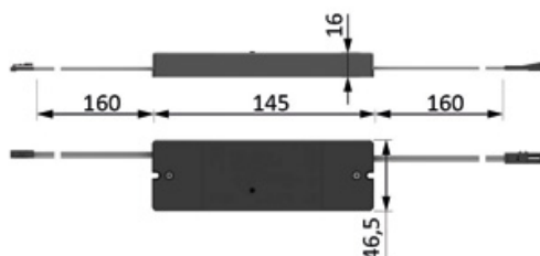
Smartempfänger des Sets 31.123.01 smart receiver of set
